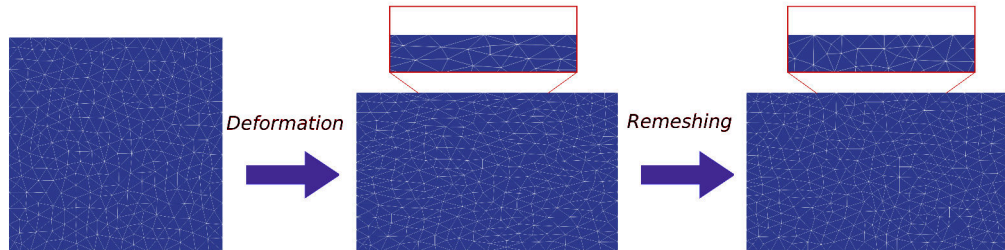
Figure 2.4: Isotropic remeshing strategy with homogeneous mesh size used in CPFEM simulations.
